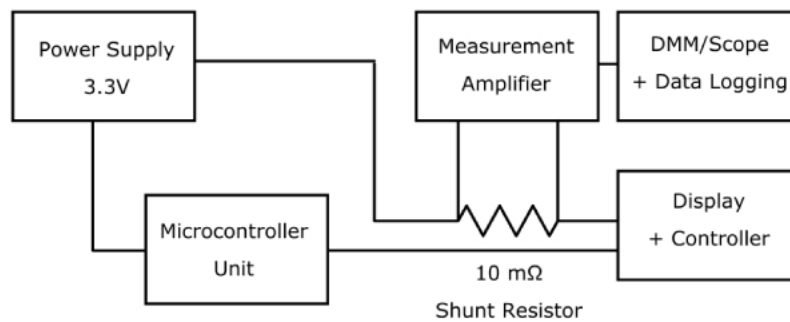
Figure 3 - Measurement Setup
