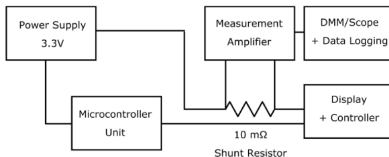
Figure 5 - Measurement Setup
